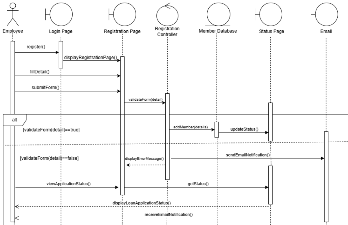
Figure 2.3.2.2: Sequence Diagram for View Membership Application Status
