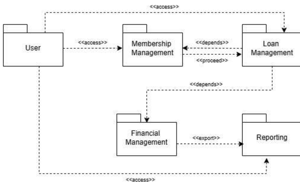
Figure 4.2.2: Package Diagram for <Koperasi KADA Online System>
