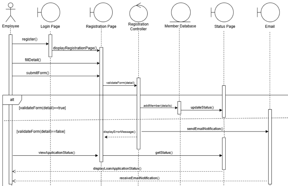
Figure 4.4.1: SD001 Sequence Diagram for <Apply Membership>
