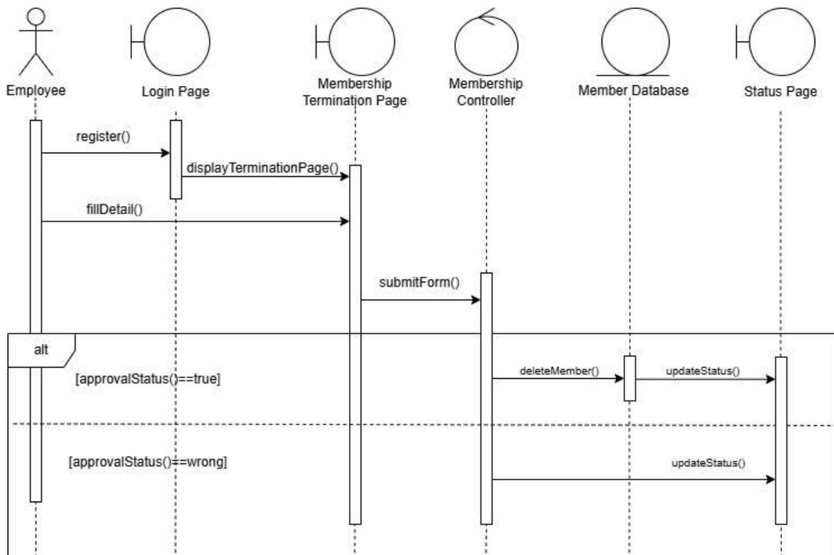
Figure 2.3.7.2: Sequence Diagram for Terminate the Membership
