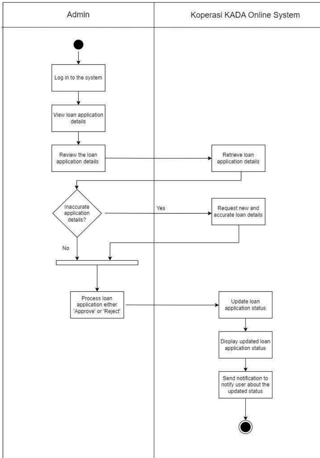
Figure 2.3.9.3: Activity Diagram for Approve Loan Application
