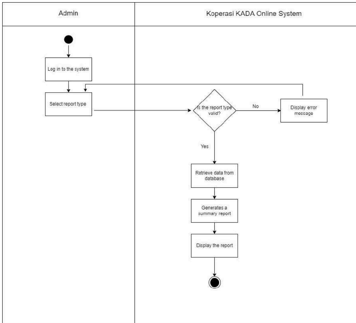
Figure 2.3.11.3: Activity Diagram for Generate Report
