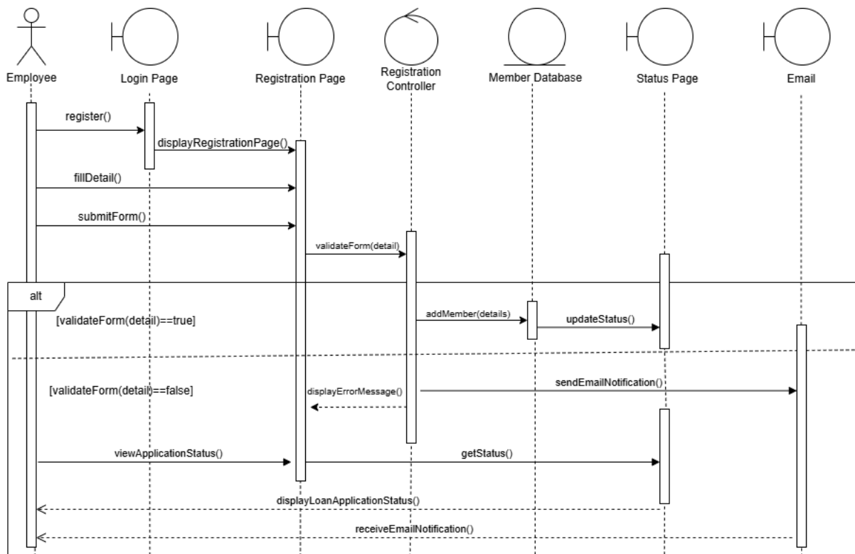
Figure 2.3.1.2: Sequence Diagram for Apply Membership
