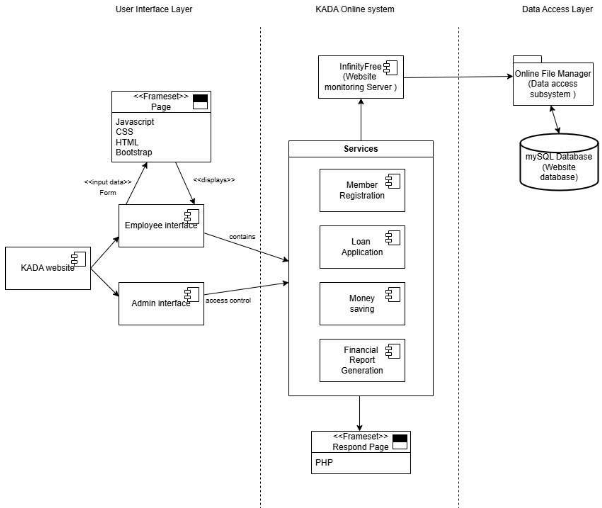
Figure 4.2.1: Architecture Diagram of <Koperasi Kada Online System>
