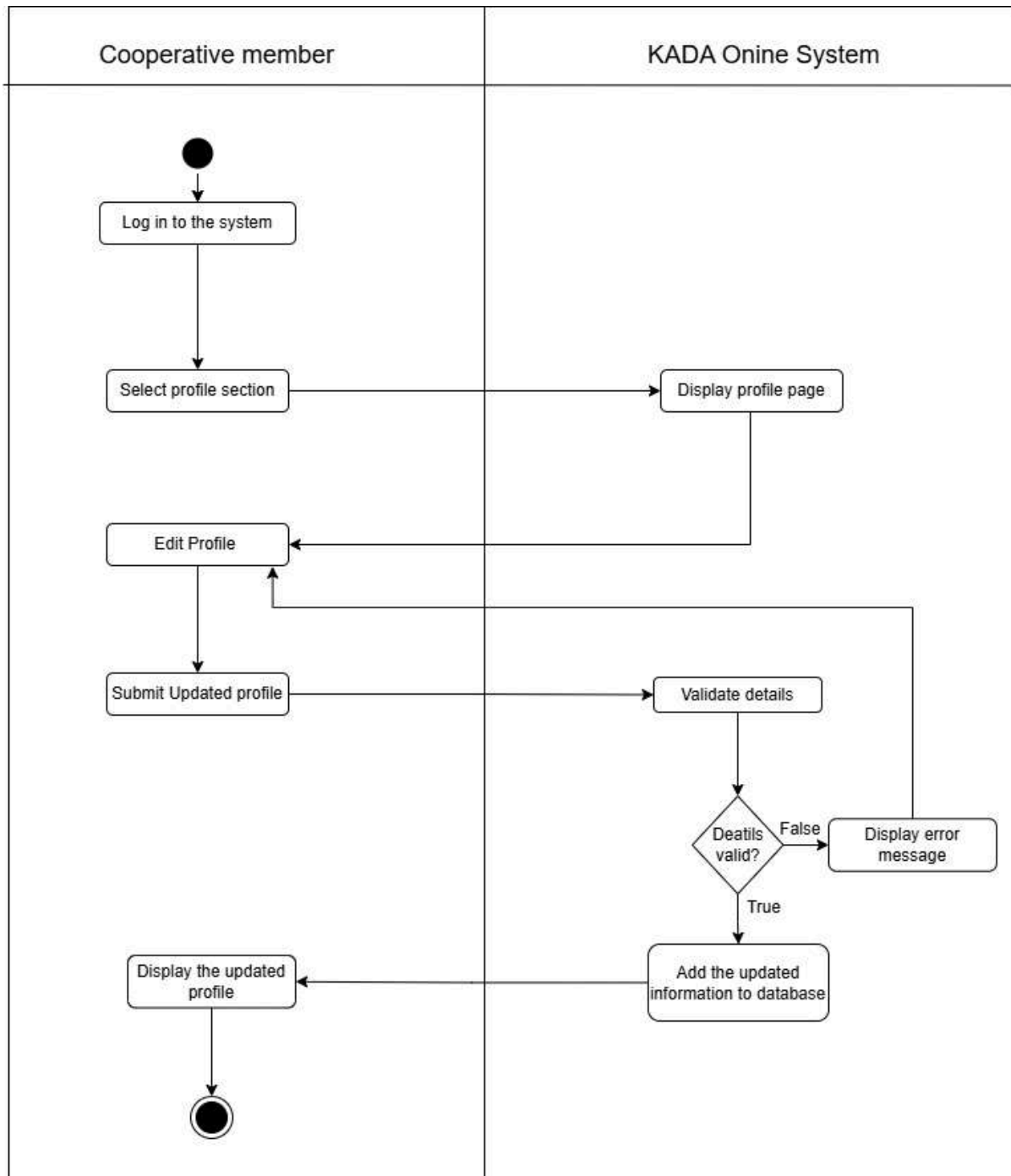
Figure 2.3.6.3: Activity Diagram for Manage Profile
