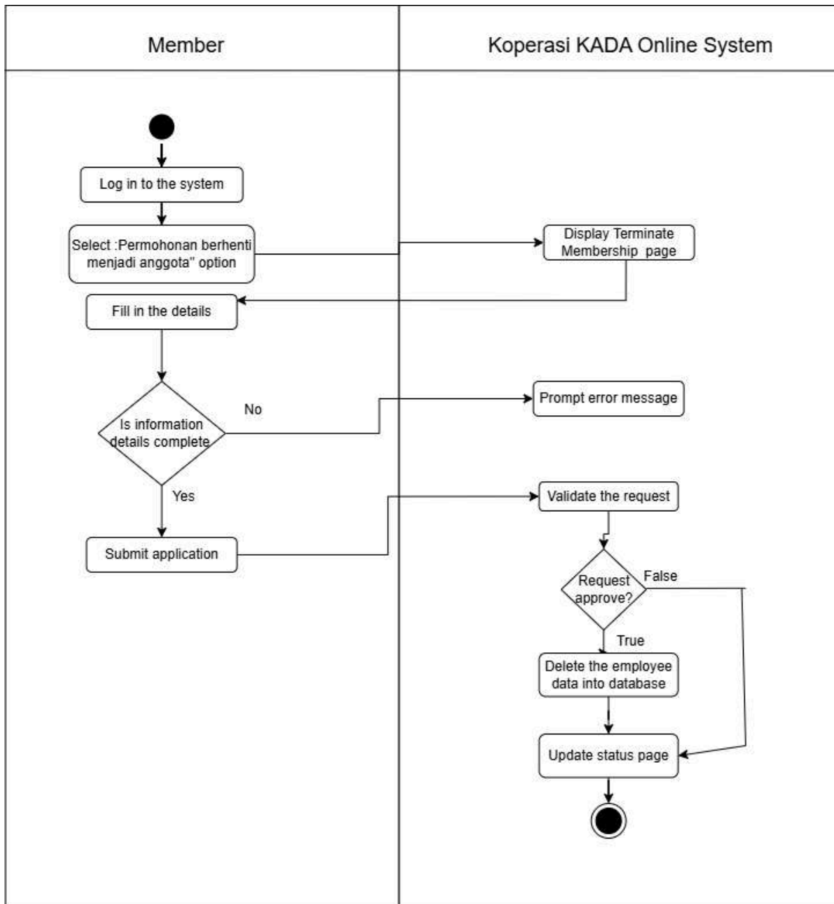
Figure 2.3.7.3: Activity Diagram for Terminate the Membership
