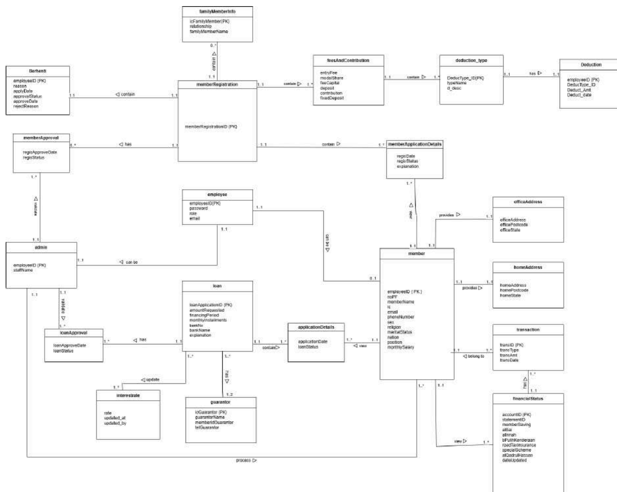
Figure 5.1 Logical ERD for Koperasi KADA Online System
