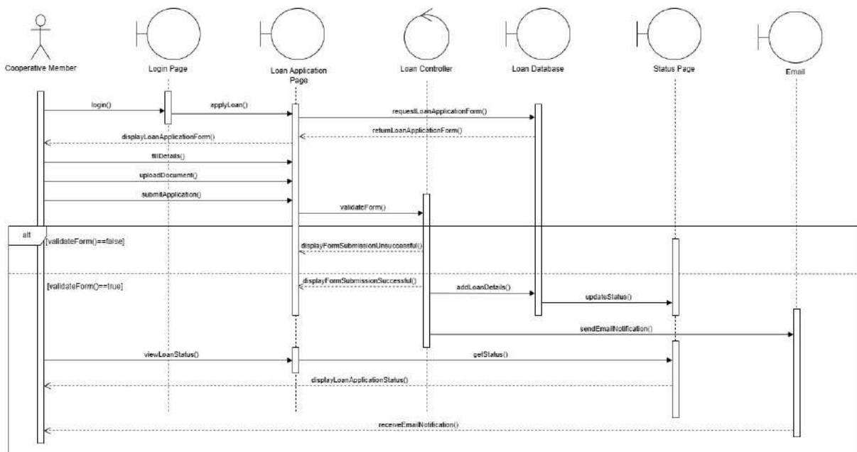
Figure 2.3.4.2: Sequence Diagram for Apply for Loan
