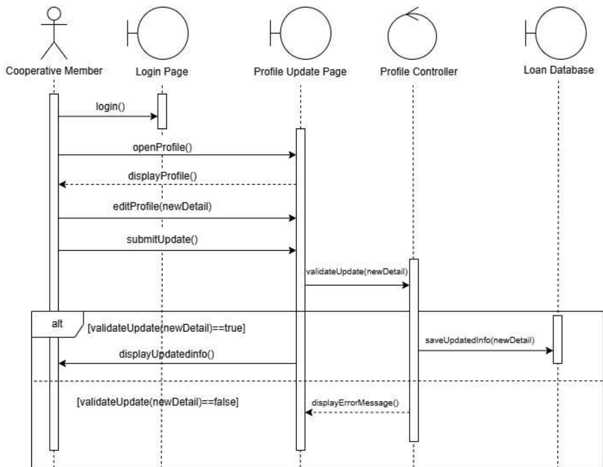
Figure 2.3.6.2: Sequence Diagram for Manage Profile
