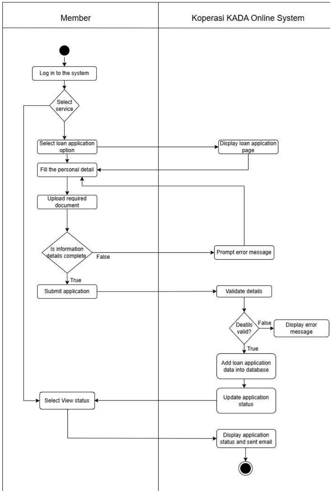
Figure 2.3.4.3: Activity Diagram for Apply for Loan
