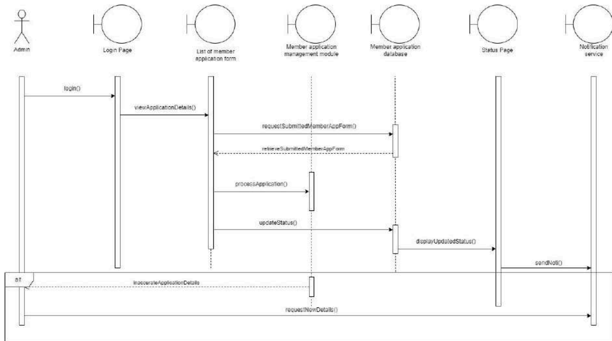
Figure 2.3.8.2: Sequence Diagram for Approve Membership Application
