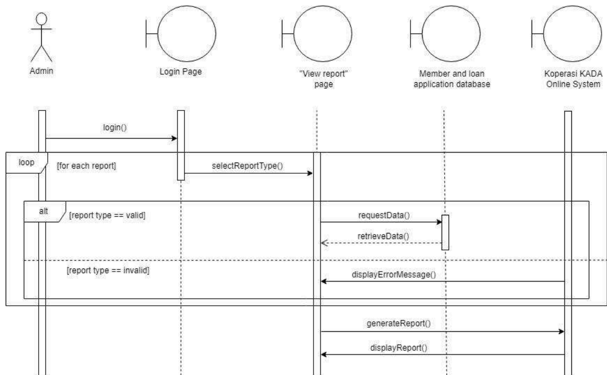
Figure 2.3.11.2: Sequence Diagram for Generate Report
