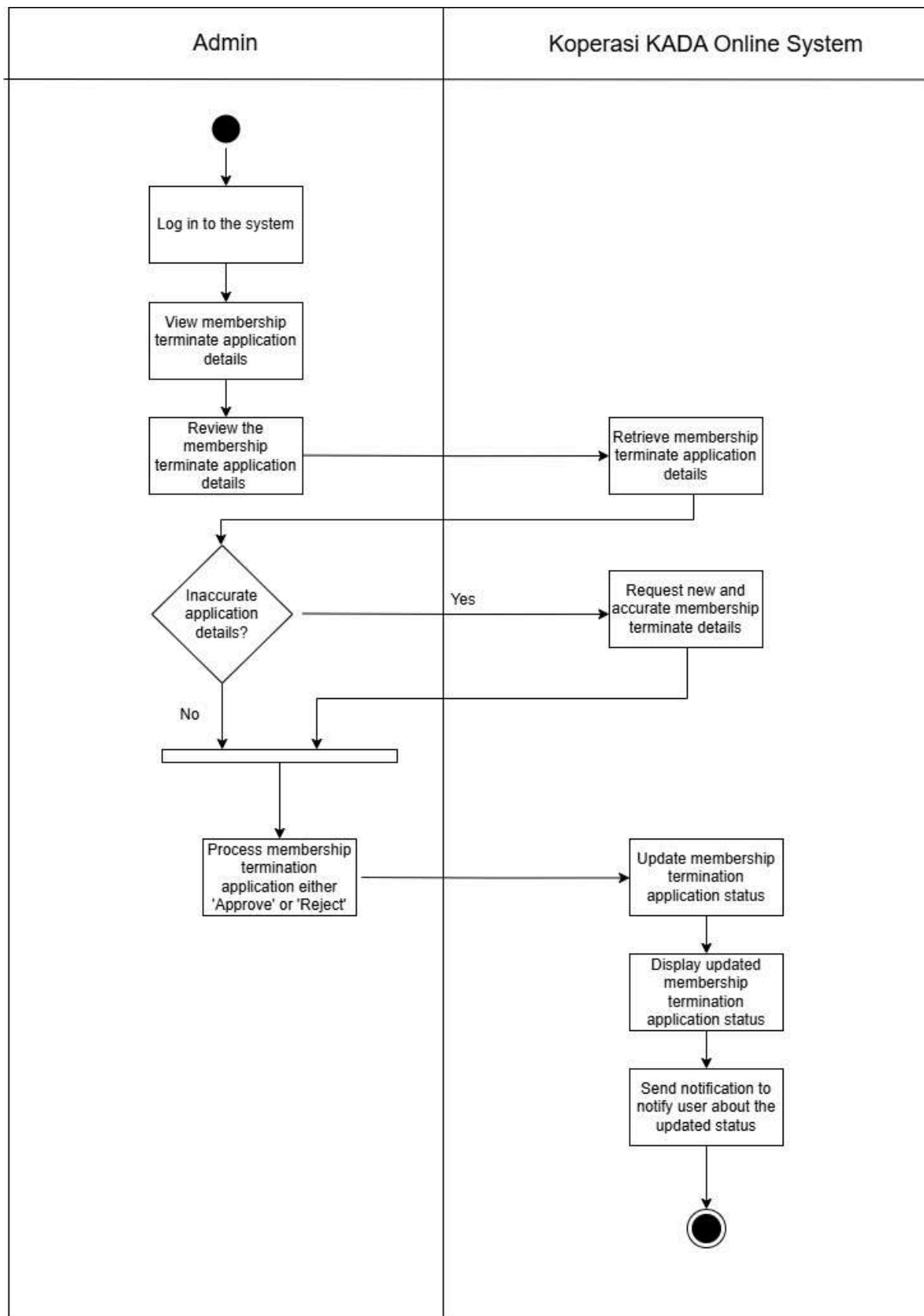
Figure 2.3.10.3: Activity Diagram for Approve Terminate Membership Application
