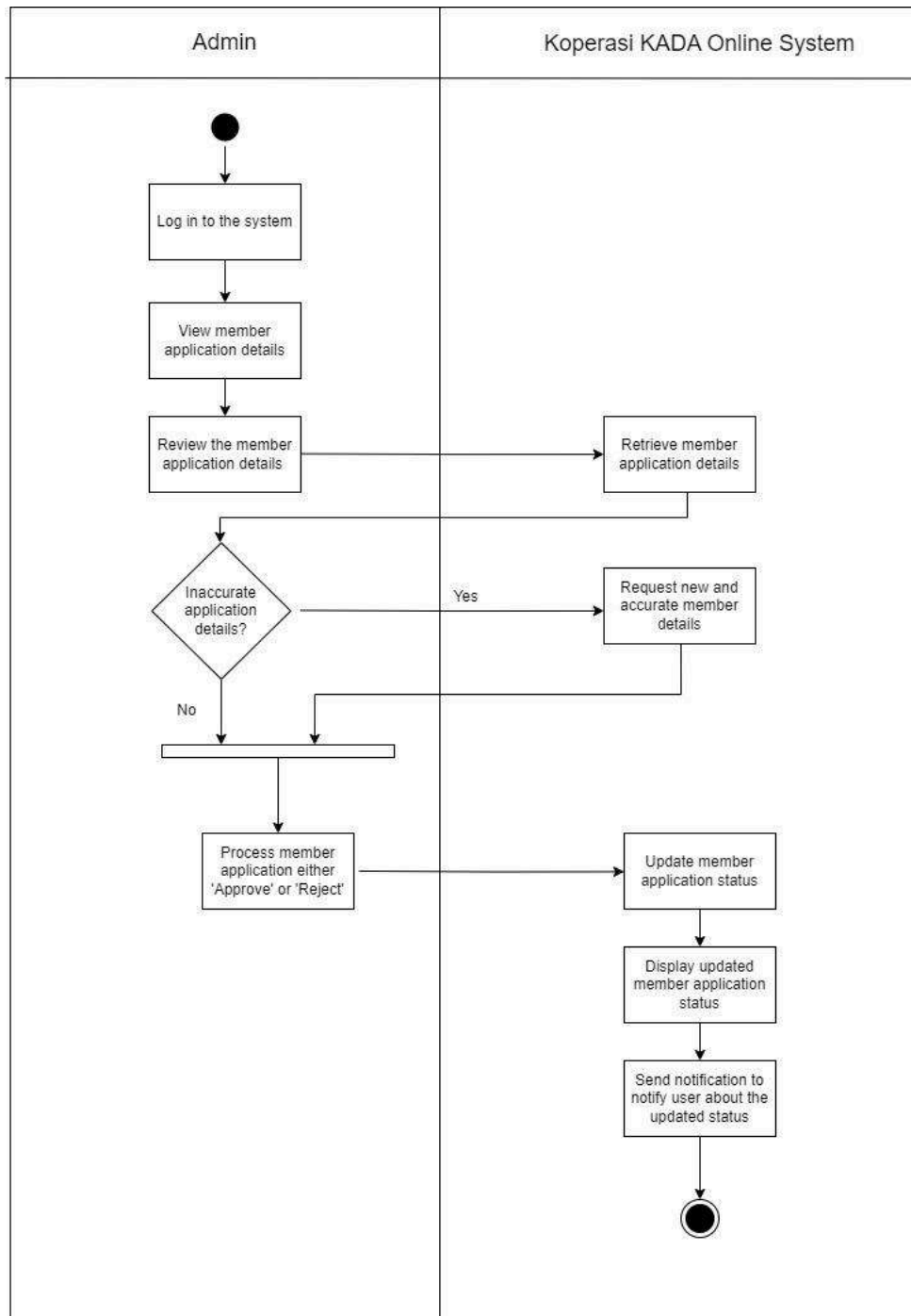
Figure 2.3.8.3: Activity Diagram for Approve Membership Application
