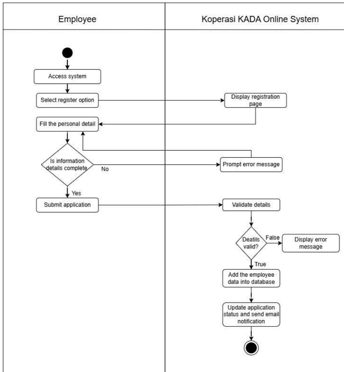
Figure 2.3.1.3: Activity Diagram for Apply Membership
