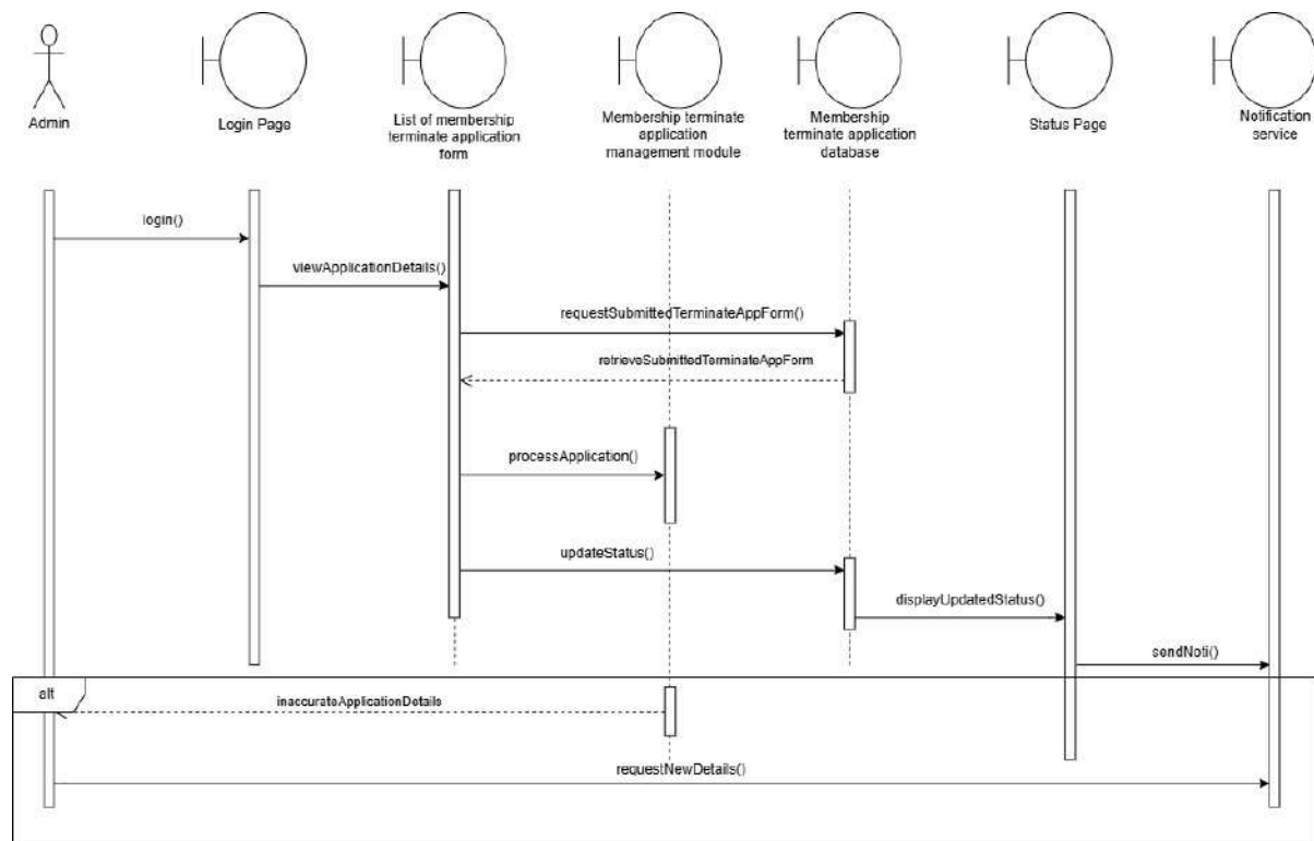
Figure 2.3.10.2: Sequence Diagram for Approve Terminate Membership Application
