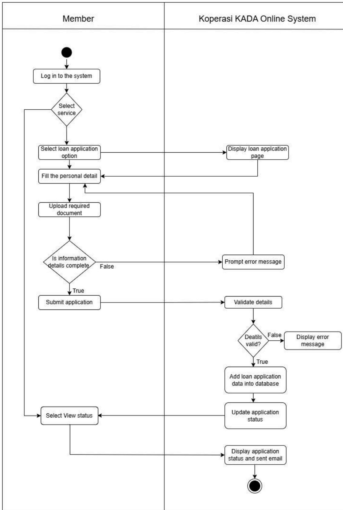
Figure 2.3.5.3: Activity Diagram for View loan application status
