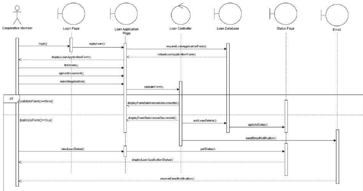
Figure 2.3.5.2: Sequence Diagram for View loan application status
