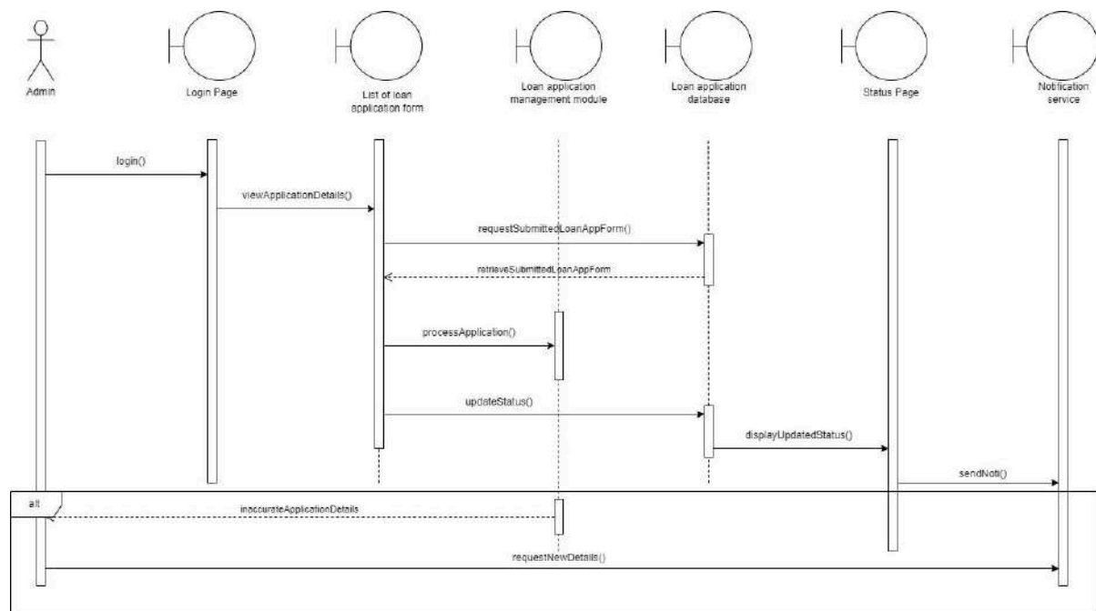
Figure 2.3.9.2: Sequence Diagram for Approve Loan Application
