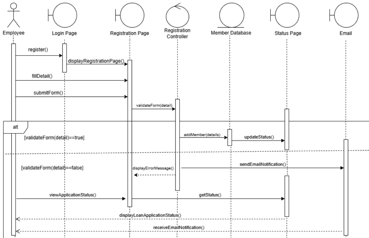
Figure 4.4.2: SD002 Sequence Diagram for <View Membership Application Status>
