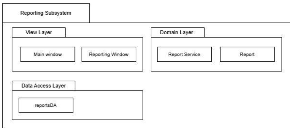
Figure 4.2.6: Package Diagram for <Reporting> Subsystem
